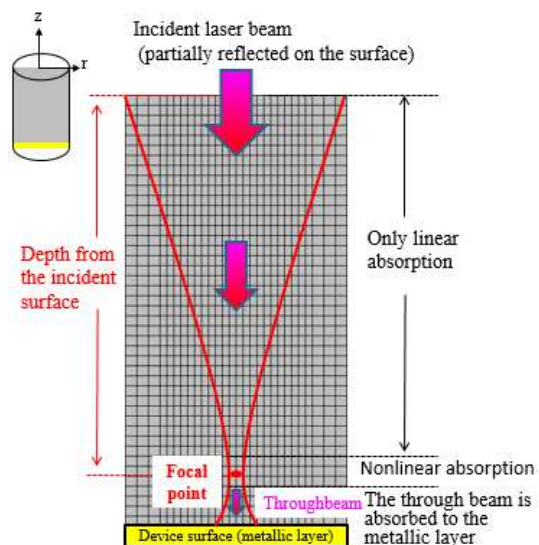
Fig.2 SD physical model
