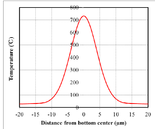
Fig.4 Radial distribution of the maximum temperature of the bottom Cu layer
